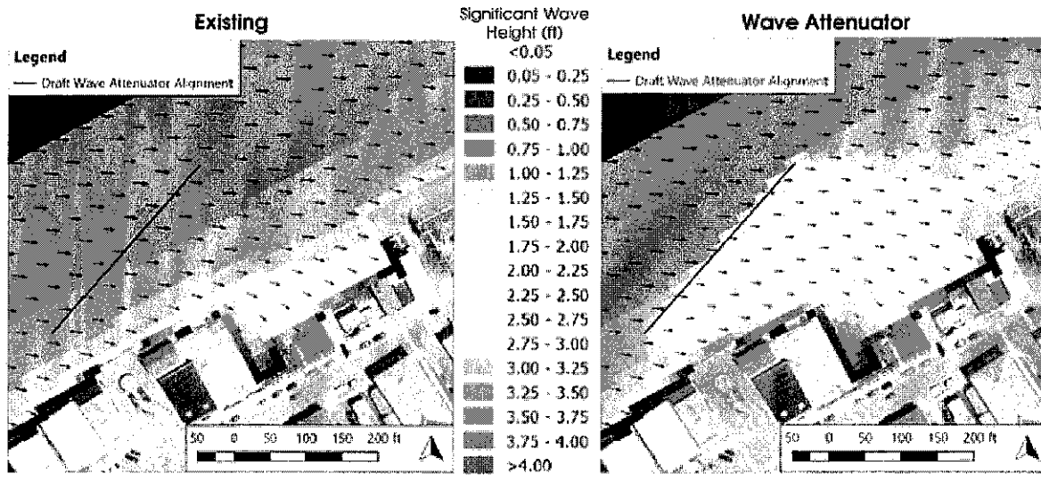
Model simulation showing the effects of adding a floating wave attenuator along a developed shoreline
